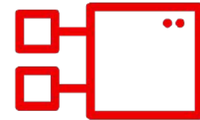
Microservices Architecture
